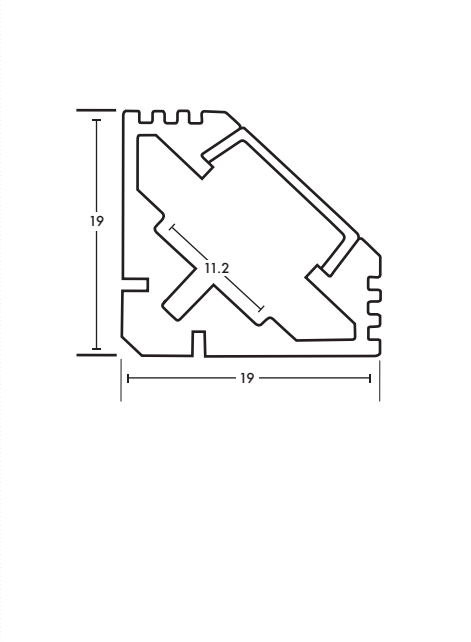
Corner Mounted Flexible Tape Extrusion - EXT4
