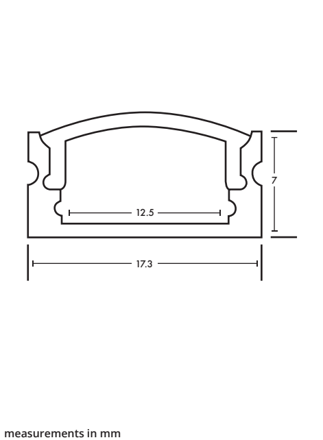
Surface Mounted Flexible Tape Extrusion - EXT1
