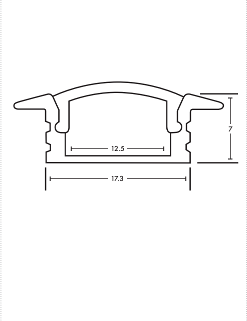
Recessed Mounted Flexible Tape Extrusion - EXT3
